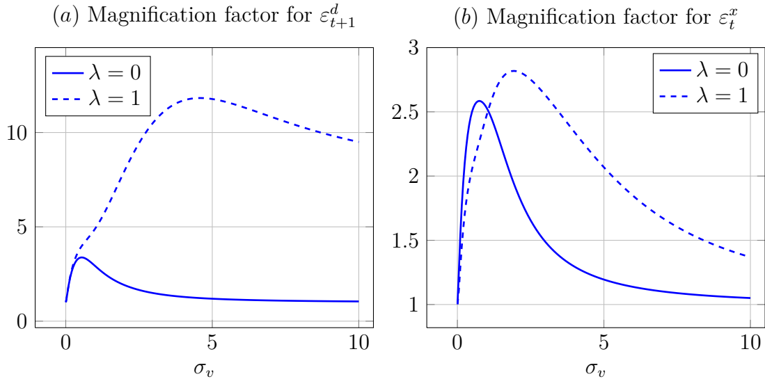
Figure 6: Magnification Factors.
