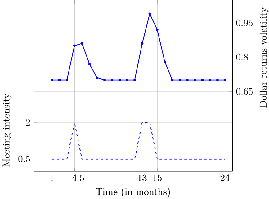
Figure 9: Volatility Clustering.
